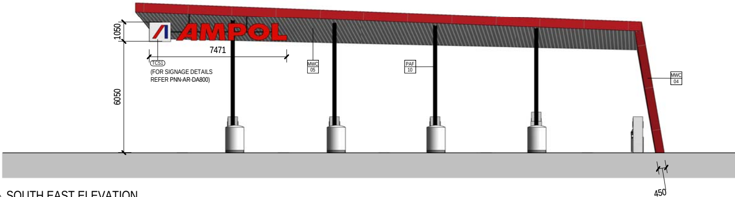
1 SOUTH EAST ELEVATION A101 1 : 100 @ A1
