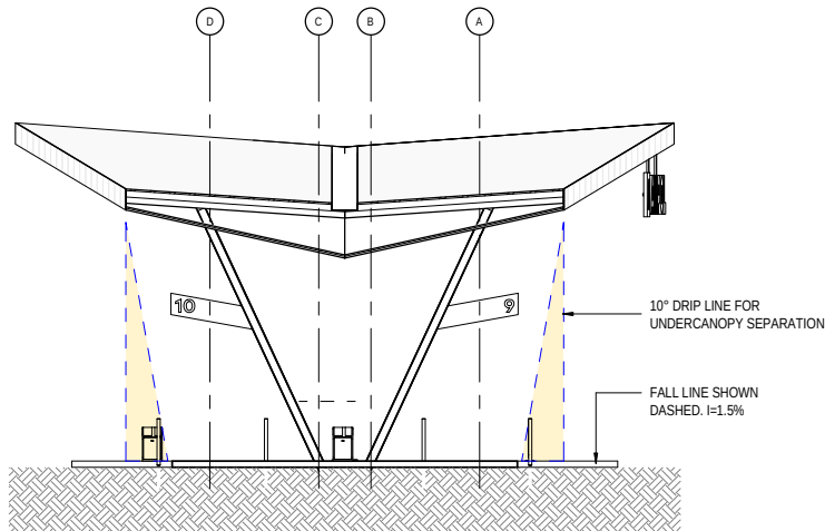
2 CAR CANOPY SECTION 02 1 : 100 @ A1
