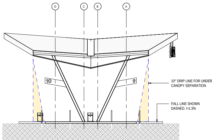
1 CAR CANOPY SECTION 02 1 : 100 @ A1
