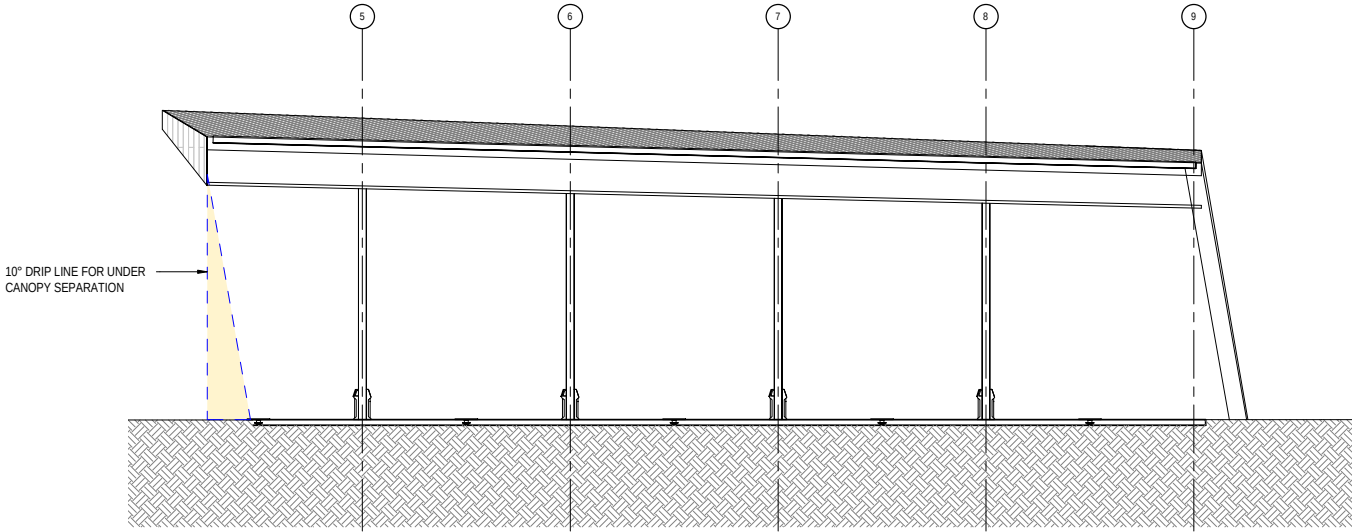
1 TRUCKS CANOPY SECTION 01 1 : 100 @ A1
