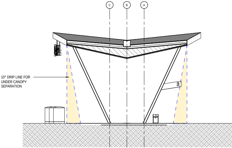
2 PNN-TRUCKS CANOPY SECTION - 1 : 100 @ A1
