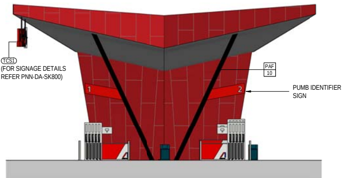
4 SOUTH WEST ELEVATION DA082S 1 : 100 @ A1
