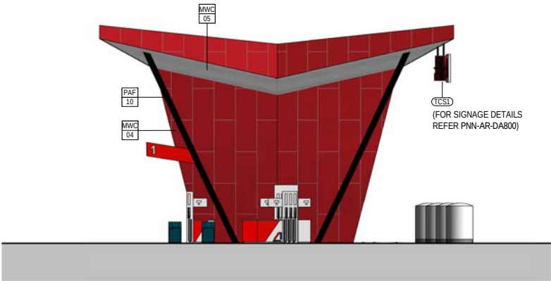
3 SOUTH WEST ELEVATION A101 1 : 100 @ A1
