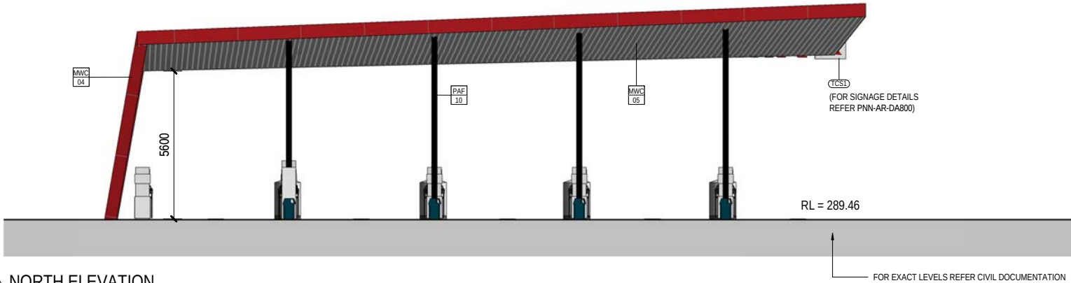
4 NORTH ELEVATION A101 1 : 100 @ A1
