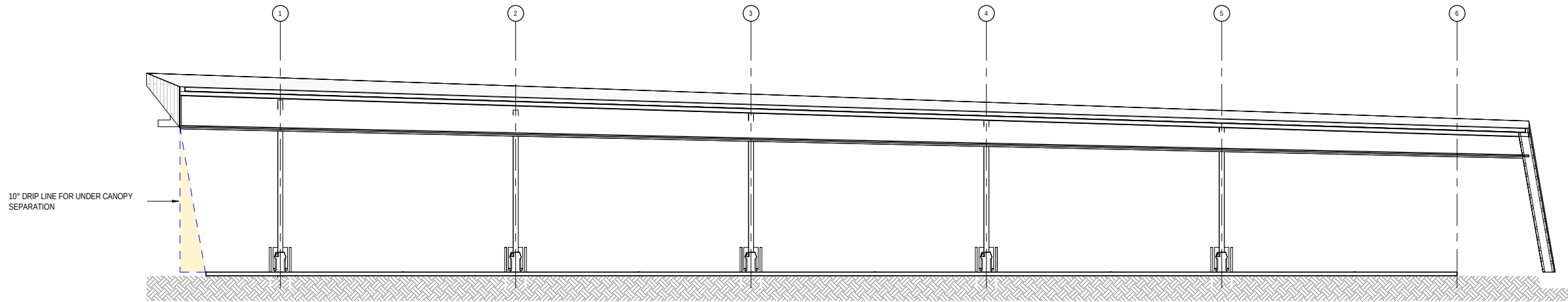
1 CAR CANOPY SECTION 01 1 : 100 @ A1
